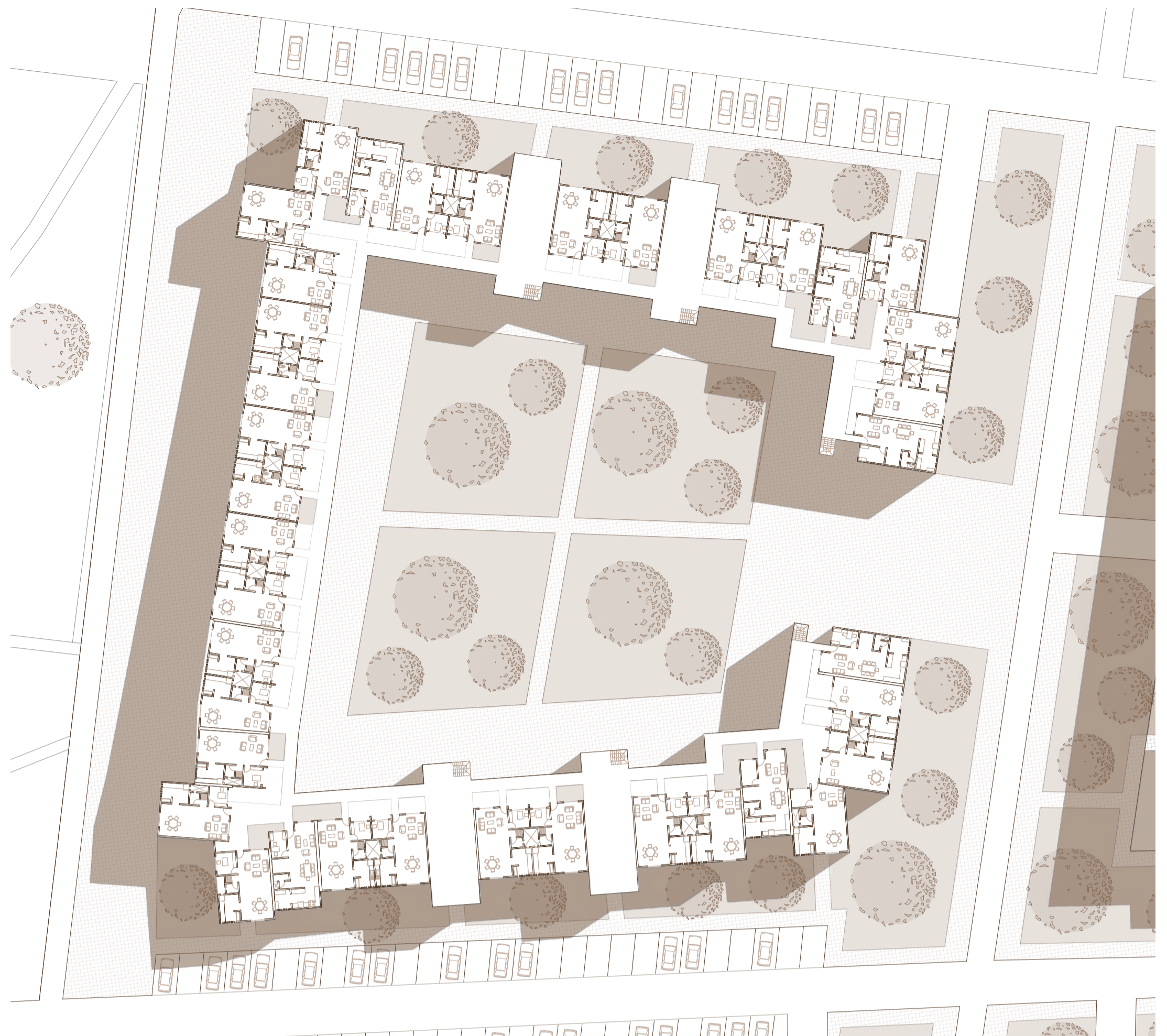
Plan residential building Scale : 1/500
